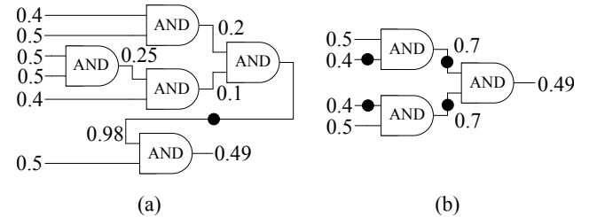
Figure 5: Synthesizing combinational logic to generate probability 0.49. (a): The circuit synthesized through Algorithm 1. (b): The circuit synthesized based on fraction factorization.
